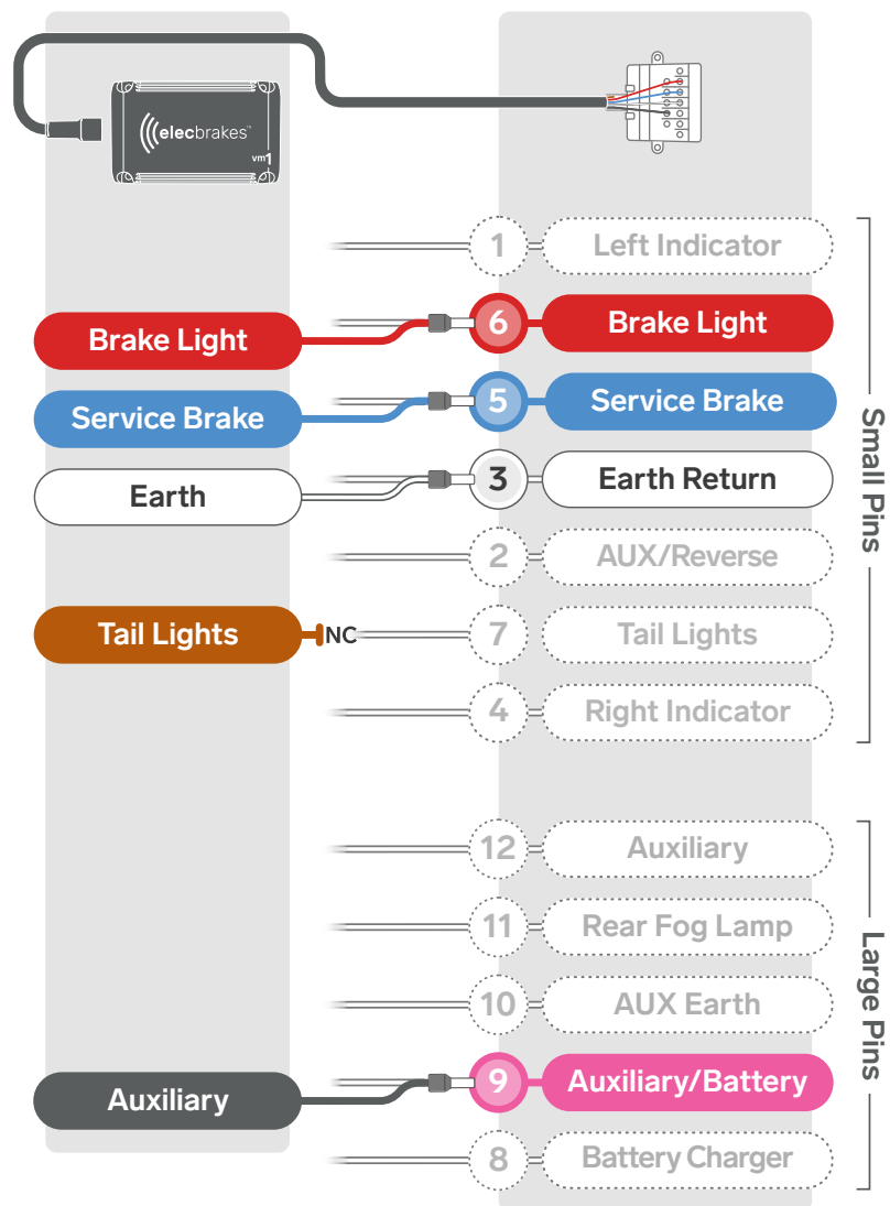
12-pin wiring diagram
