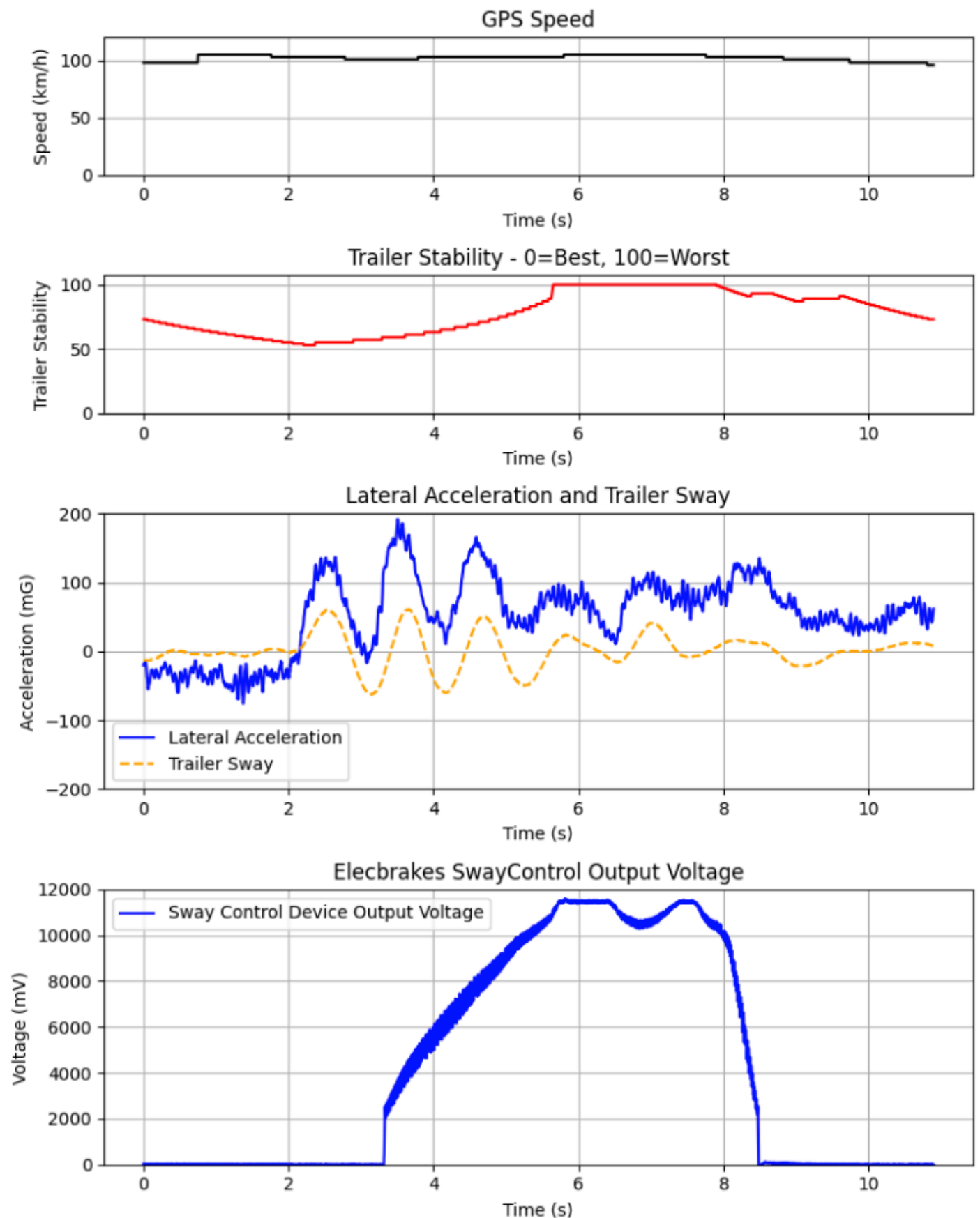
Figure 1 - Elecbrakes SwayControl performance during sway event
